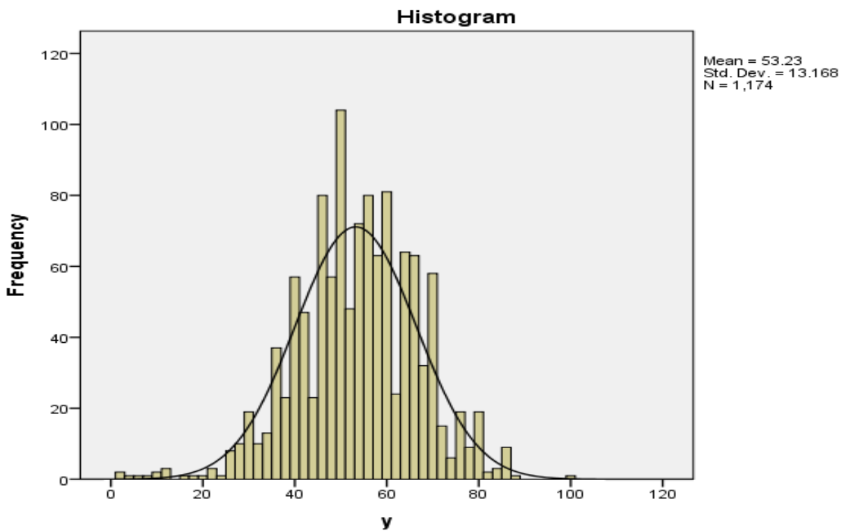
Figure 1: Normal Curve Depicting Data Distribution
